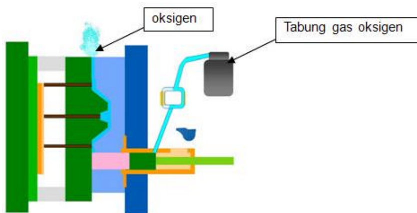
ilustrasi metode pore free casting
